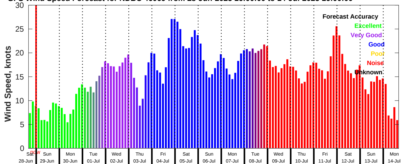
GFS Wind Speed Forecast for NDBC 46069 from 28-Jun-2025 16:00:00 to 14-Jul-2025 16:00:00
