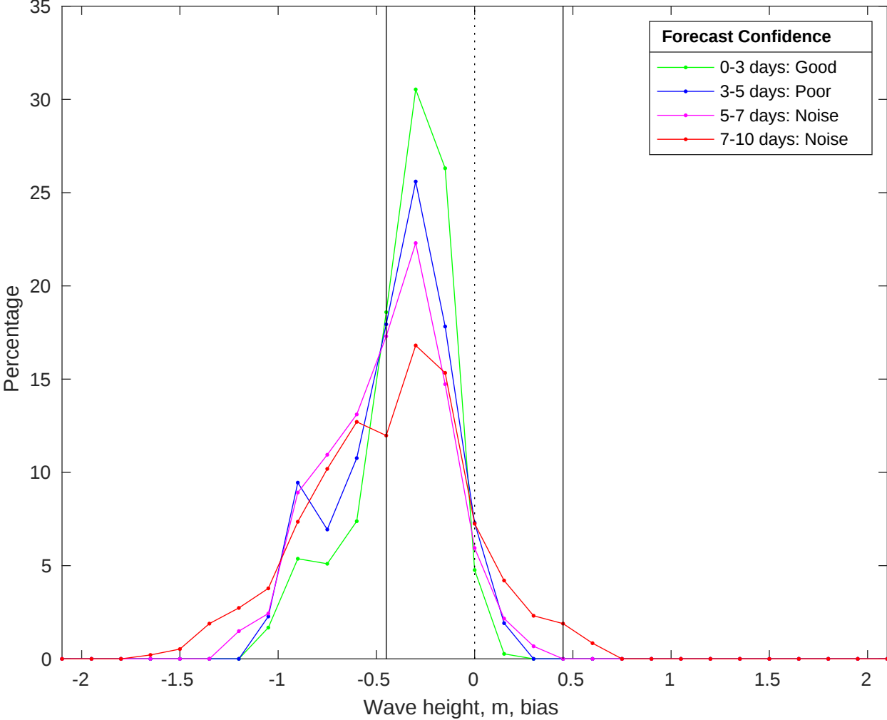
NDBC 51209 vs CMEMS Waves Bias Histogram: 29-Jun-2025
