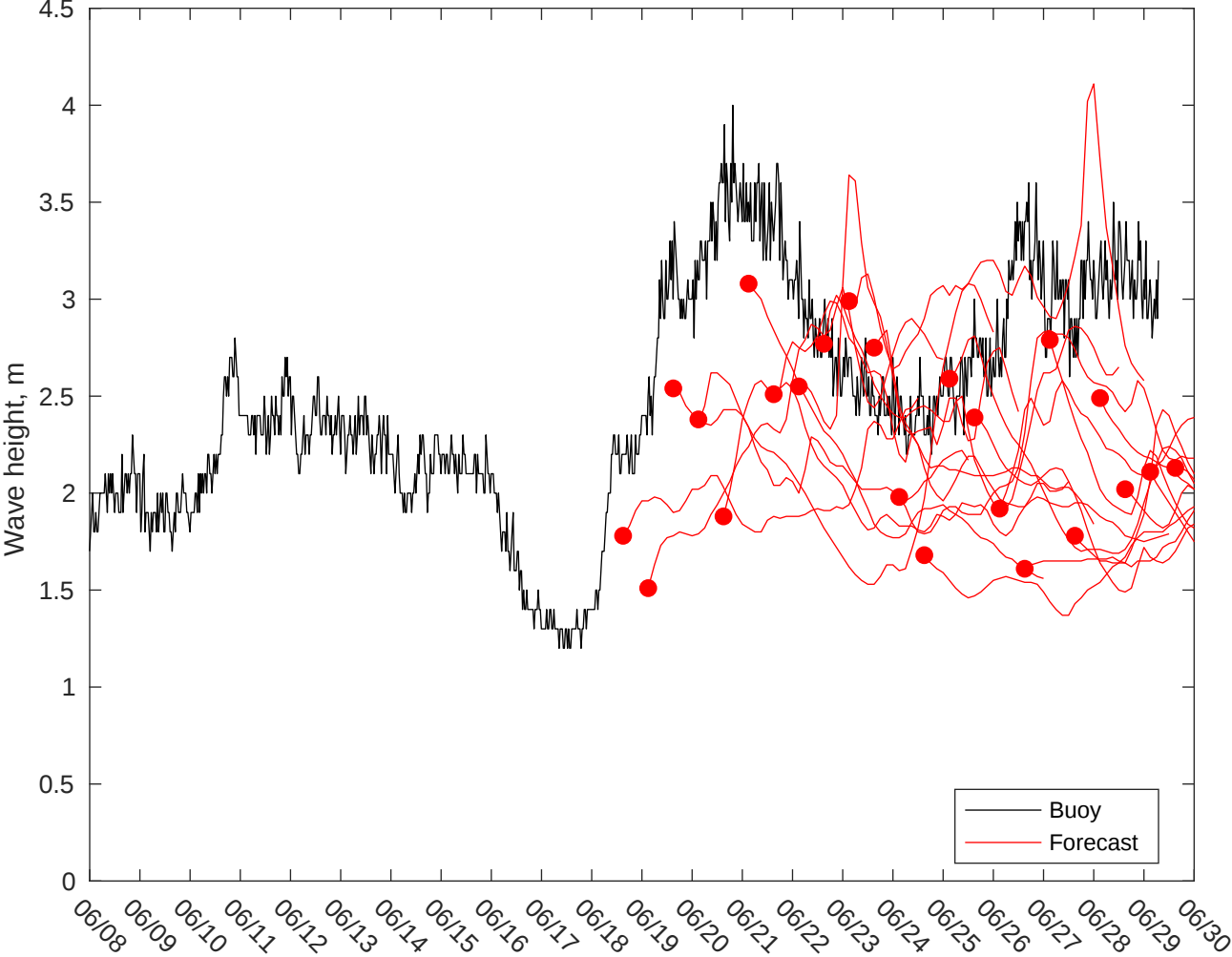
NDBC 51209 vs GFS Waves: 10 to 16 day forecast
