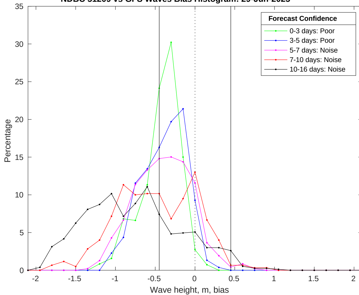
NDBC 51209 vs GFS Waves Bias Histogram: 29-Jun-2025
