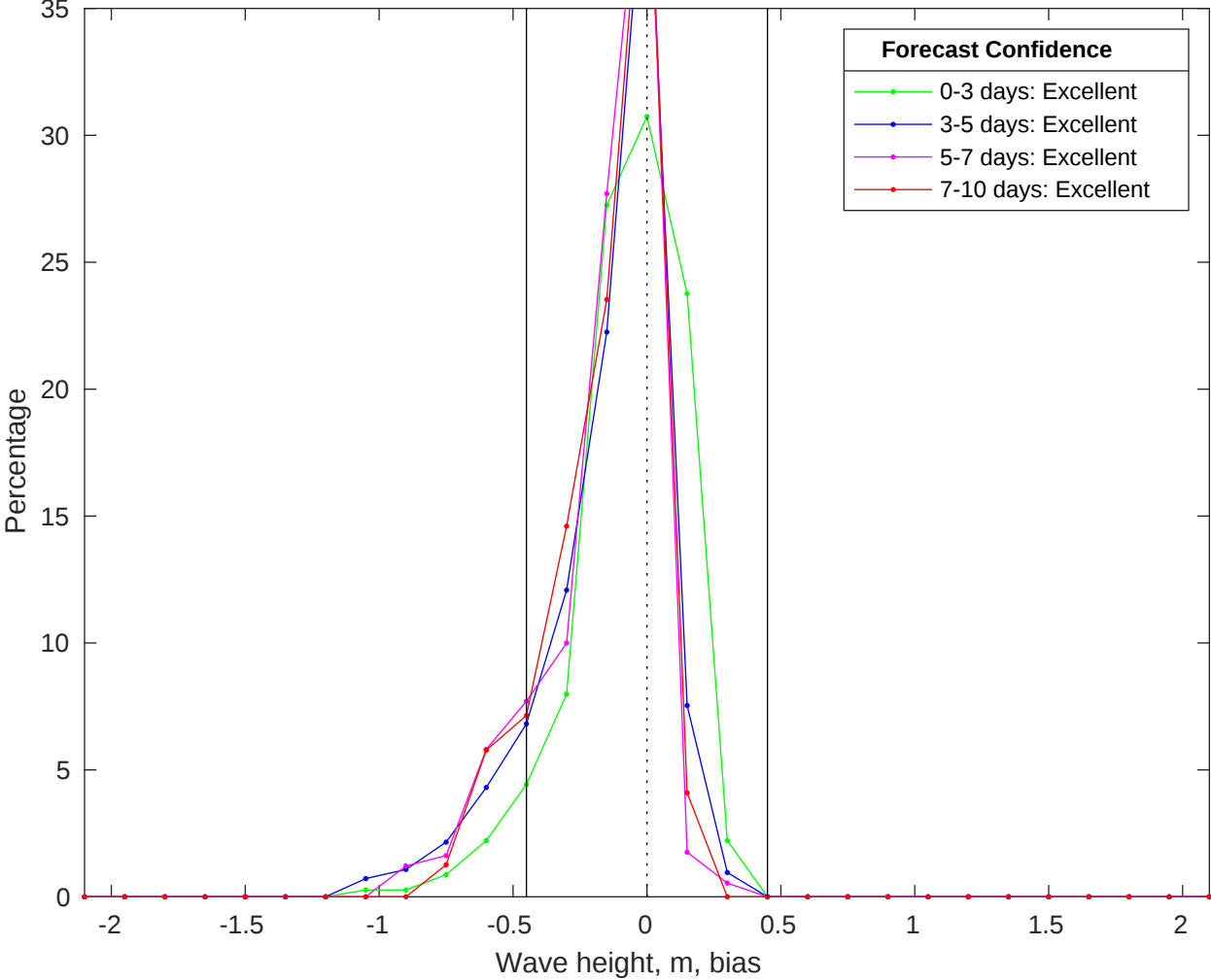
NDBC 52212 vs CMEMS Waves Bias Histogram: 29-Jun-2025
