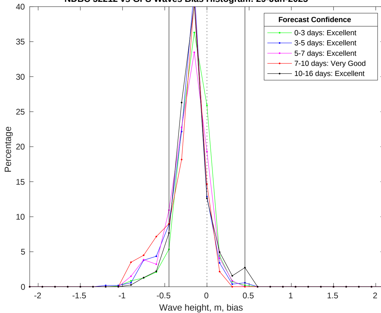
NDBC 52212 vs GFS Waves Bias Histogram: 29-Jun-2025
