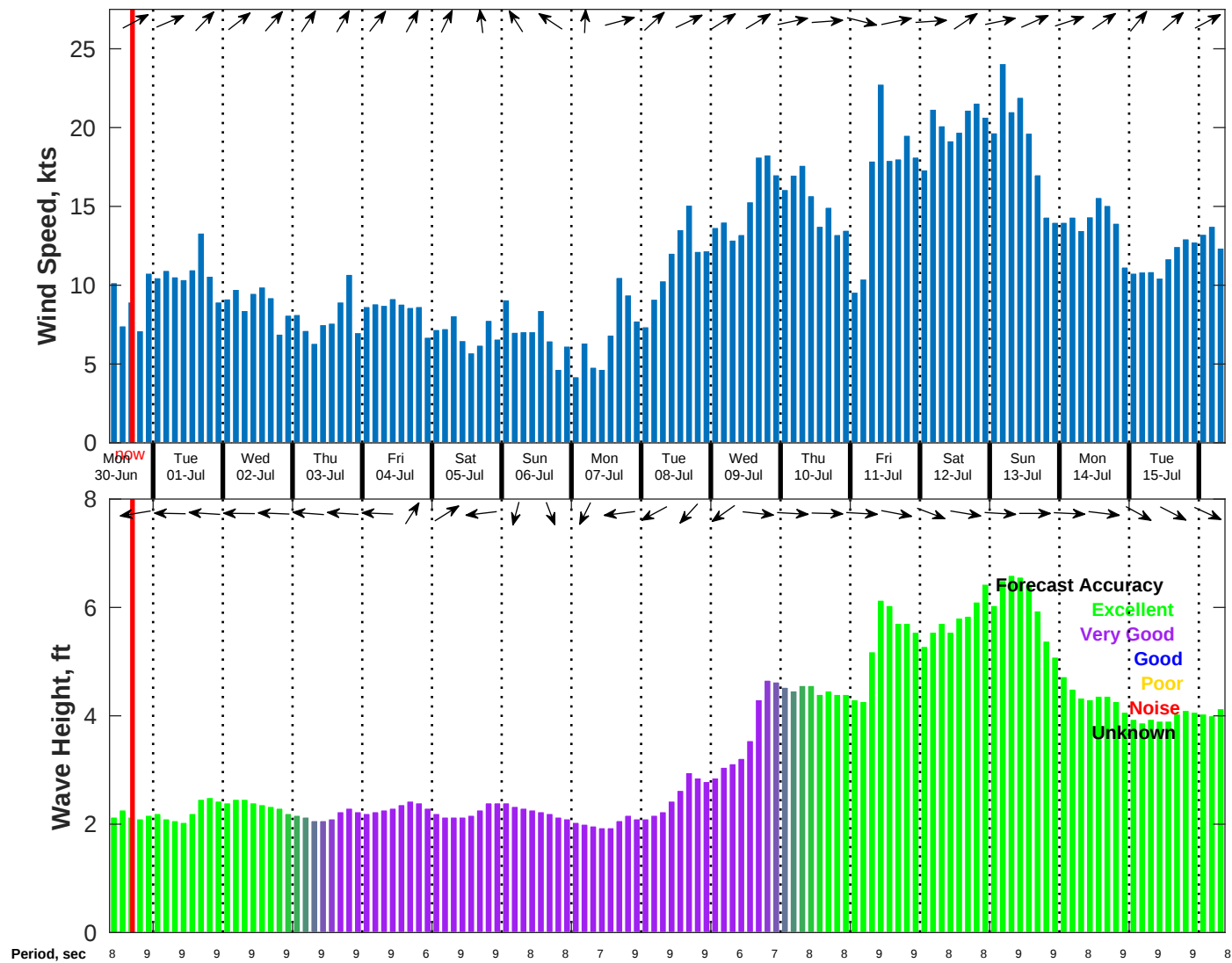
Wind & Wave Forecast for NDBC 52212 from 29-Jun-2025 09:00:00 to 15-Jul-2025 09:00:00
