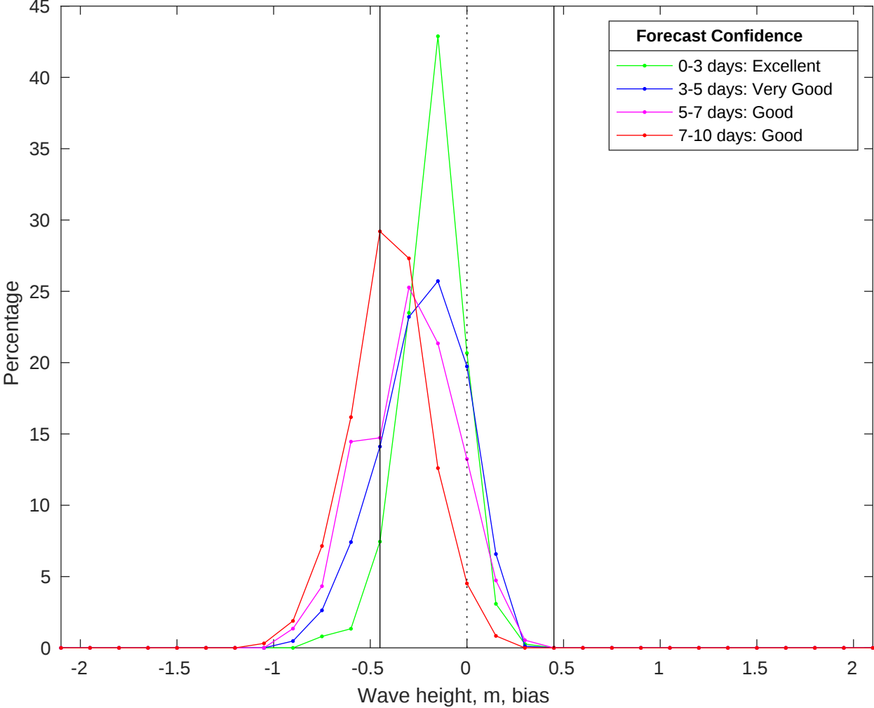
NDBC 52213 vs CMEMS Waves Bias Histogram: 29-Jun-2025
