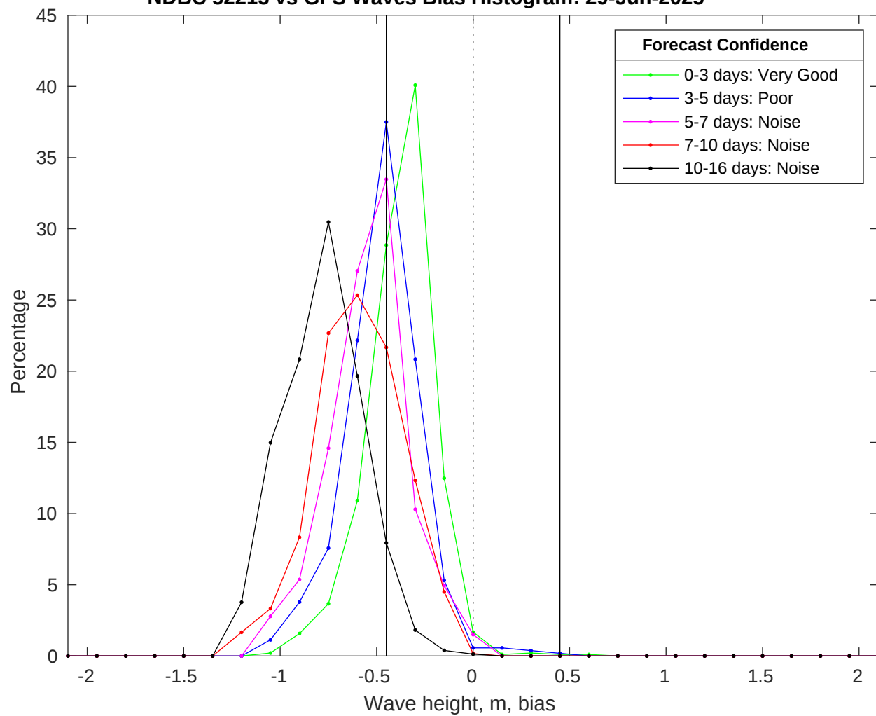
NDBC 52213 vs GFS Waves Bias Histogram: 29-Jun-2025
