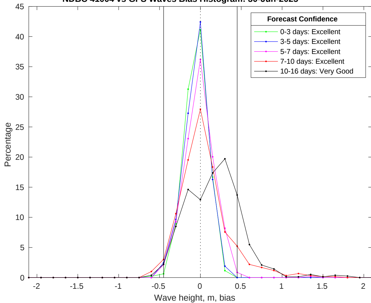
NDBC 41004 vs GFS Waves Bias Histogram: 30-Jun-2025
