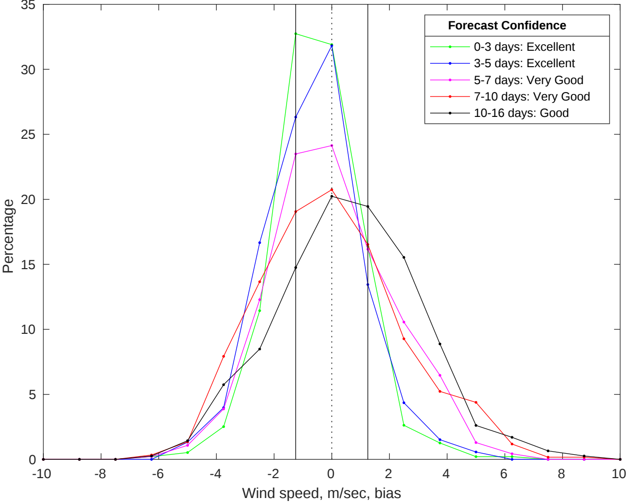
NDBC 41004 vs GFS Winds Bias Histogram: 30-Jun-2025
