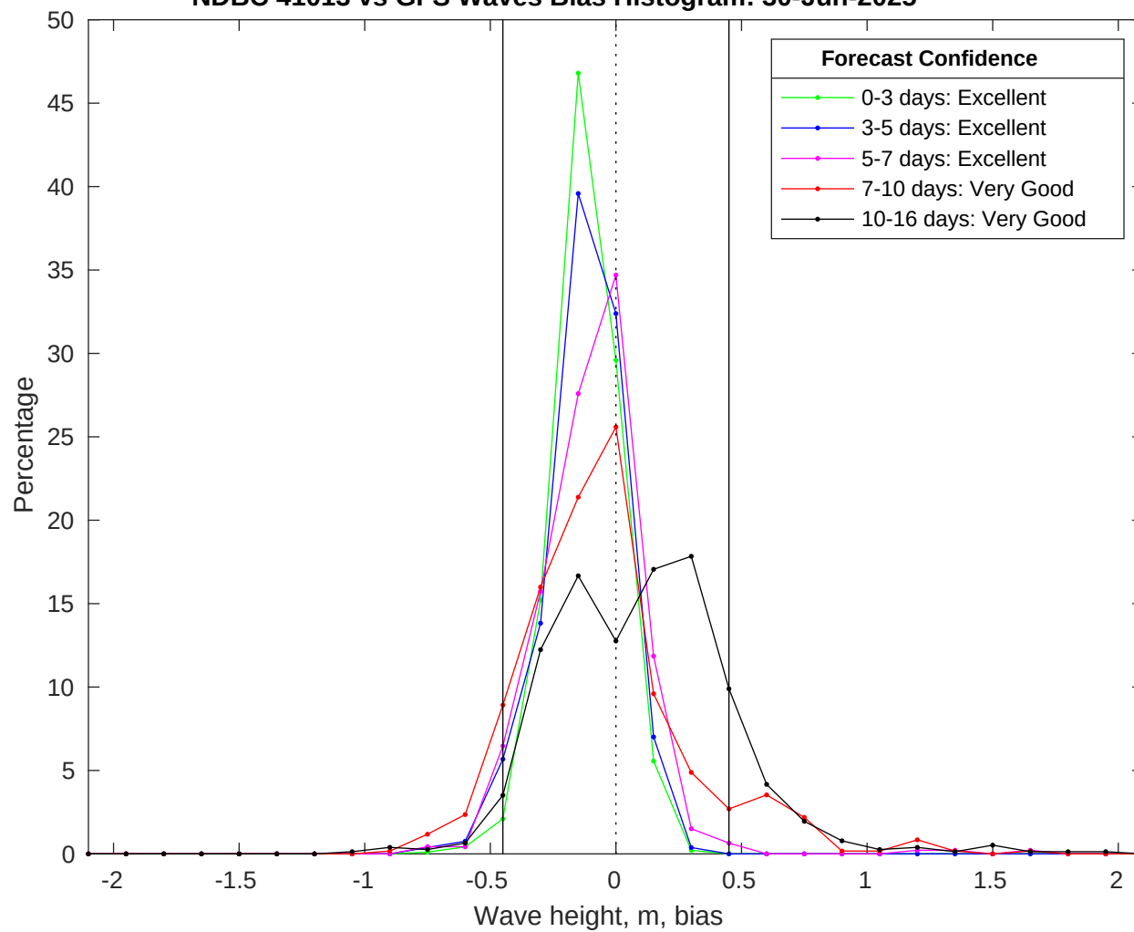
NDBC 41013 vs GFS Waves Bias Histogram: 30-Jun-2025
