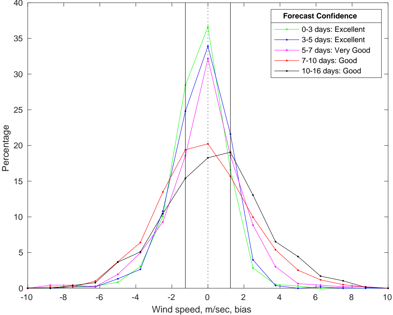
NDBC 41013 vs GFS Winds Bias Histogram: 30-Jun-2025
