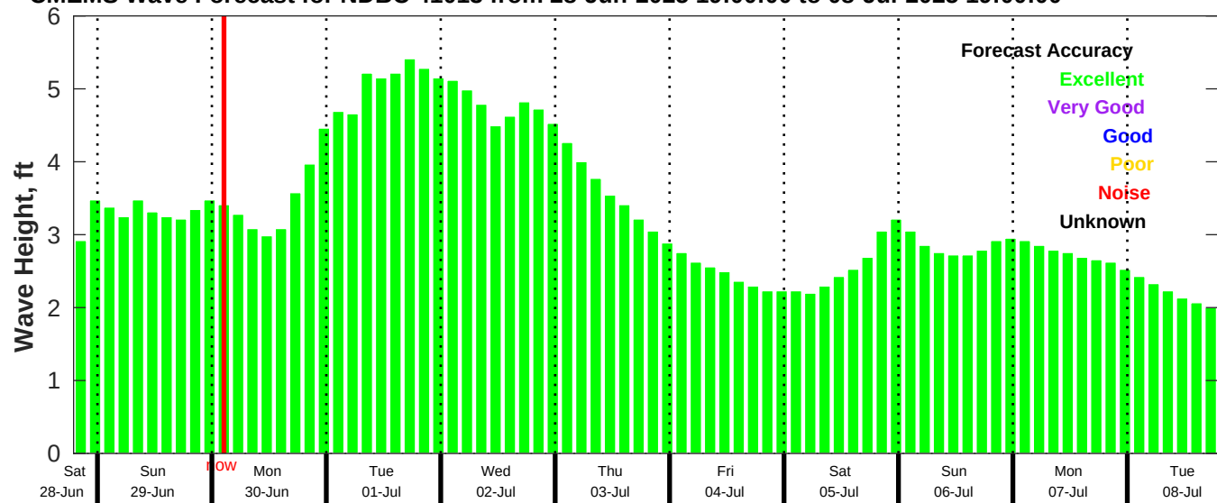
CMEMS Wave Forecast for NDBC 41013 from 28-Jun-2025 19:00:00 to 08-Jul-2025 19:00:00
