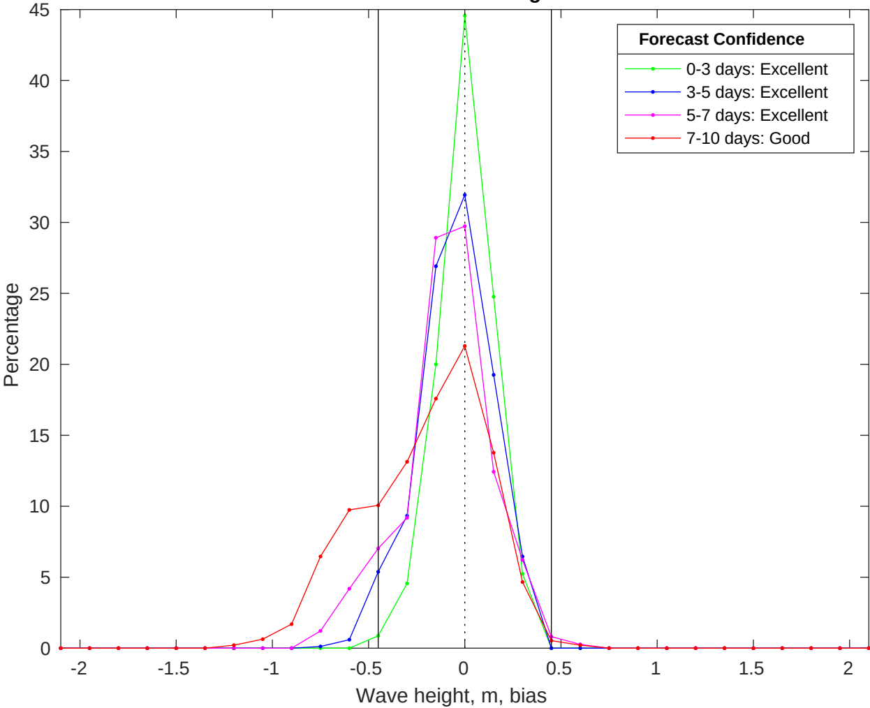
NDBC 41040 vs CMEMS Waves Bias Histogram: 30-Jun-2025
