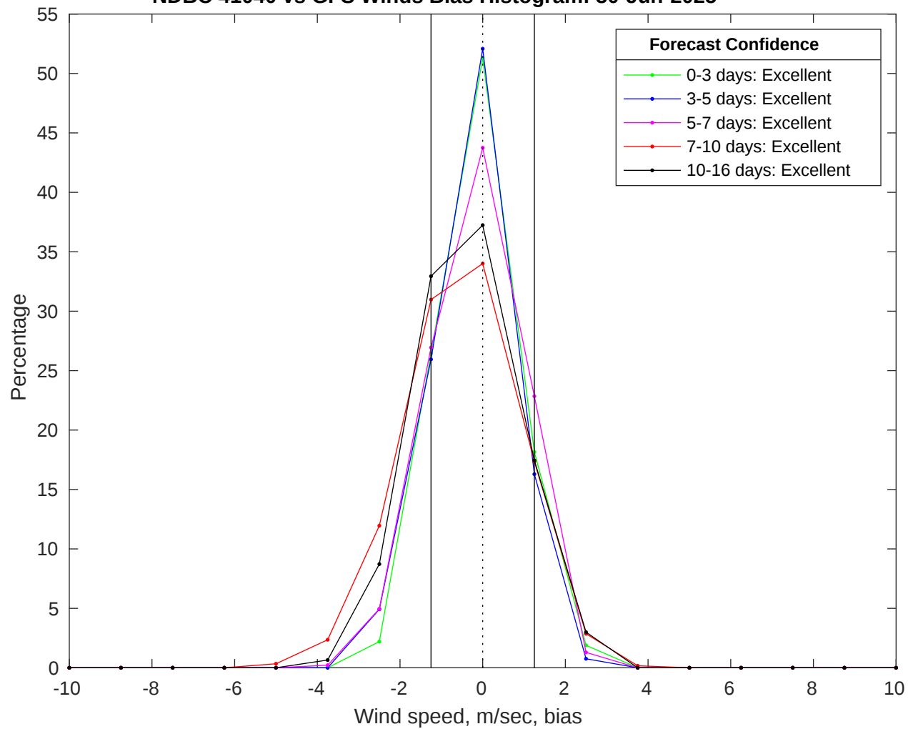
NDBC 41040 vs GFS Winds Bias Histogram: 30-Jun-2025
