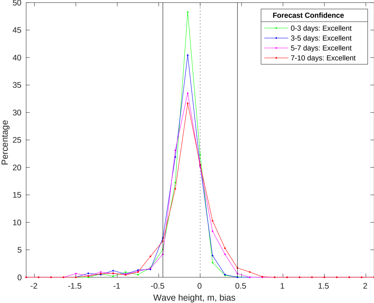
NDBC 42019 vs CMEMS Waves Bias Histogram: 30-Jun-2025
