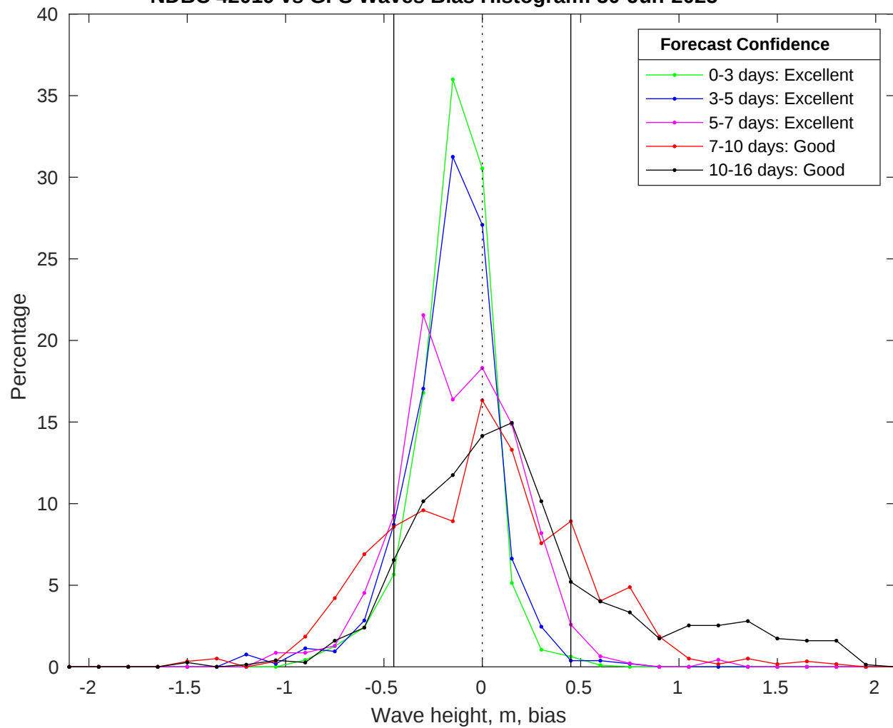
NDBC 42019 vs GFS Waves Bias Histogram: 30-Jun-2025
