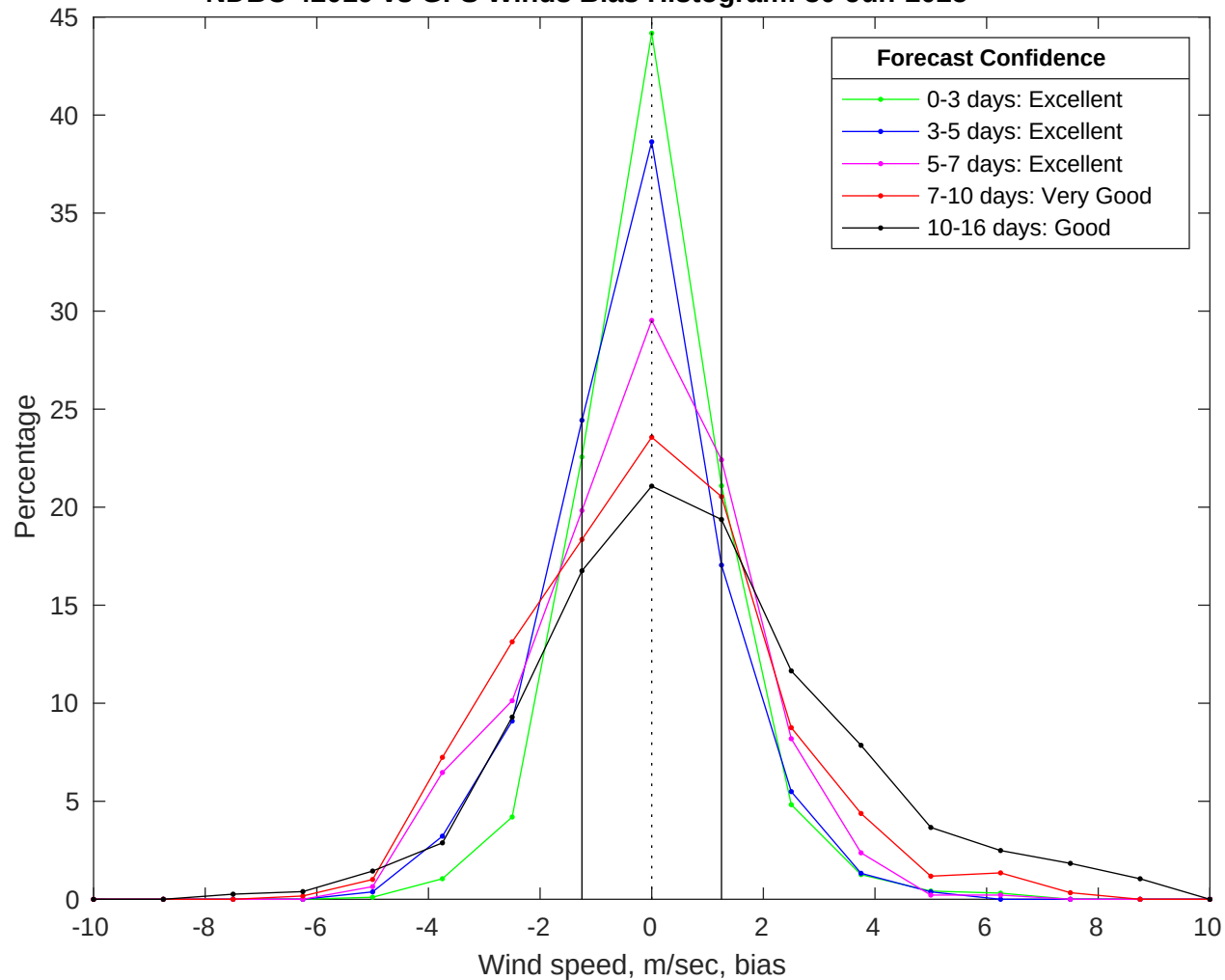
NDBC 42019 vs GFS Winds Bias Histogram: 30-Jun-2025
