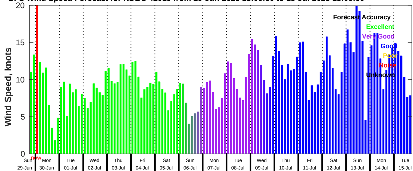
GFS Wind Speed Forecast for NDBC 42019 from 29-Jun-2025 18:00:00 to 15-Jul-2025 18:00:00
