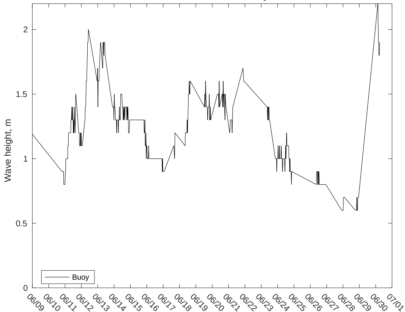
NDBC 42020 vs CMEMS Waves: 10 to 16 day forecast
