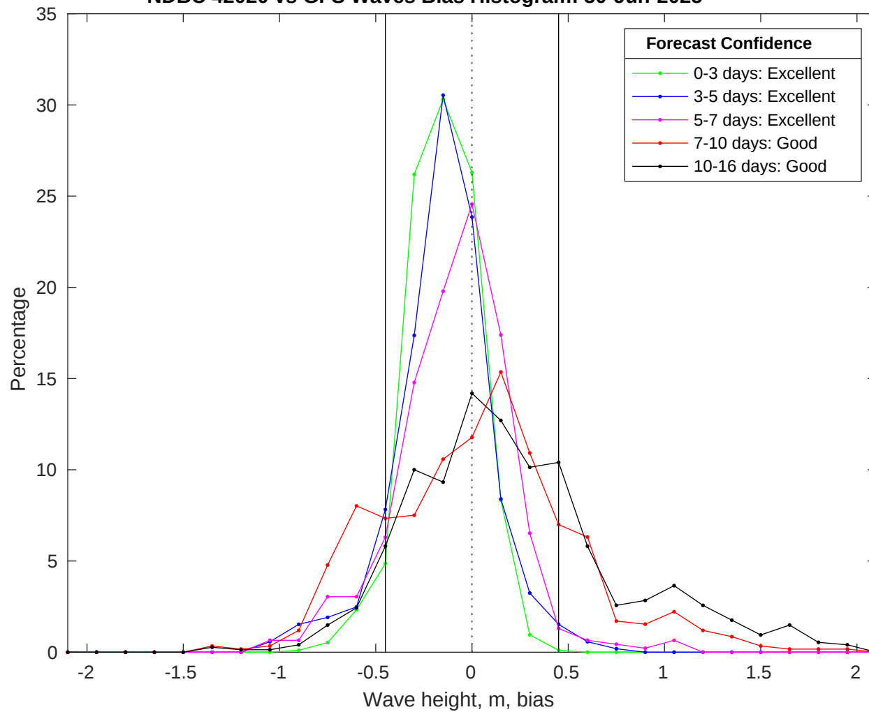
NDBC 42020 vs GFS Waves Bias Histogram: 30-Jun-2025
