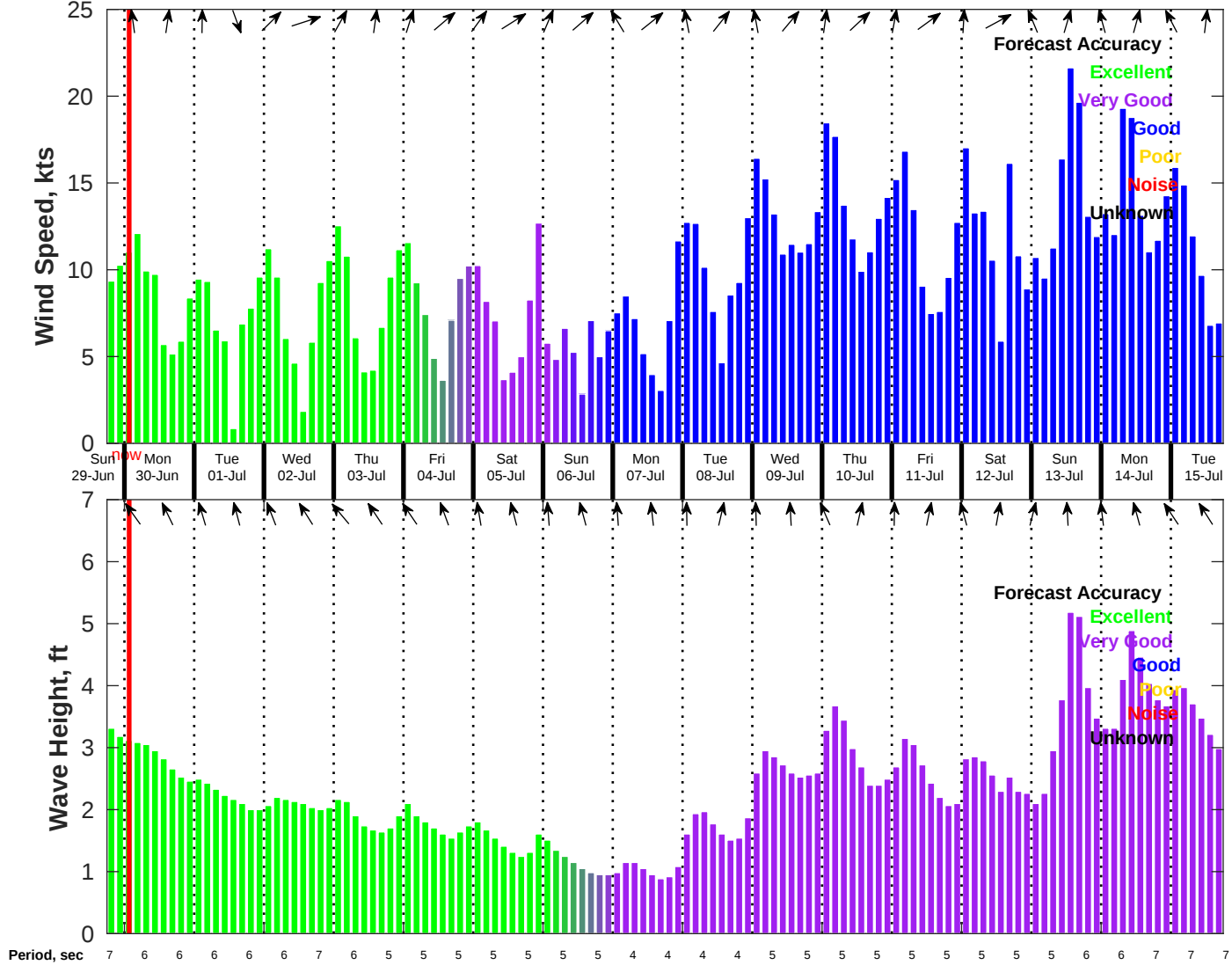
Wind & Wave Forecast for NDBC 42035 from 29-Jun-2025 18:00:00 to 15-Jul-2025 18:00:00
