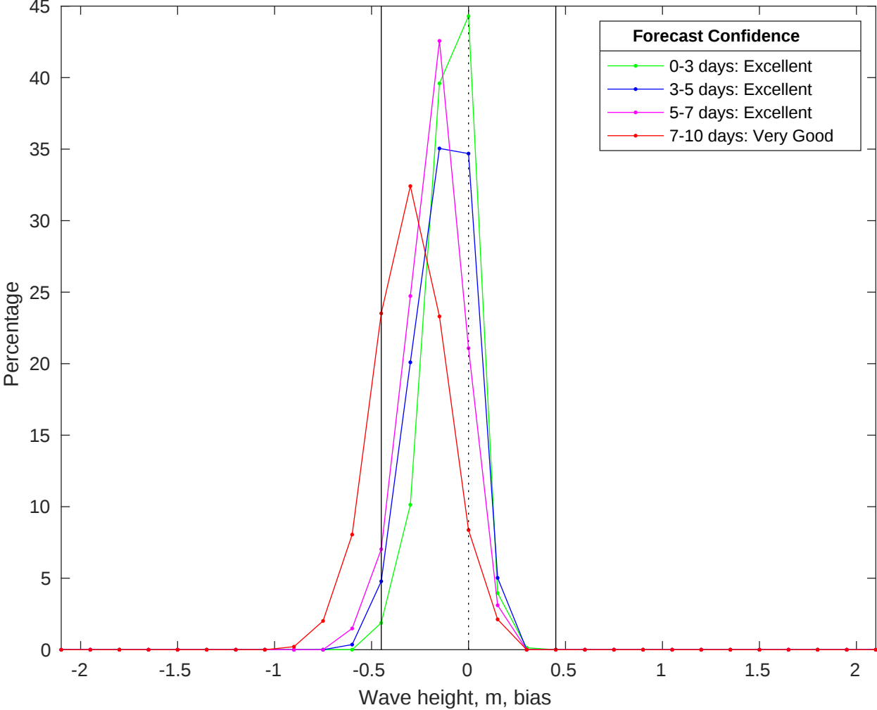
NDBC 42036 vs CMEMS Waves Bias Histogram: 30-Jun-2025
