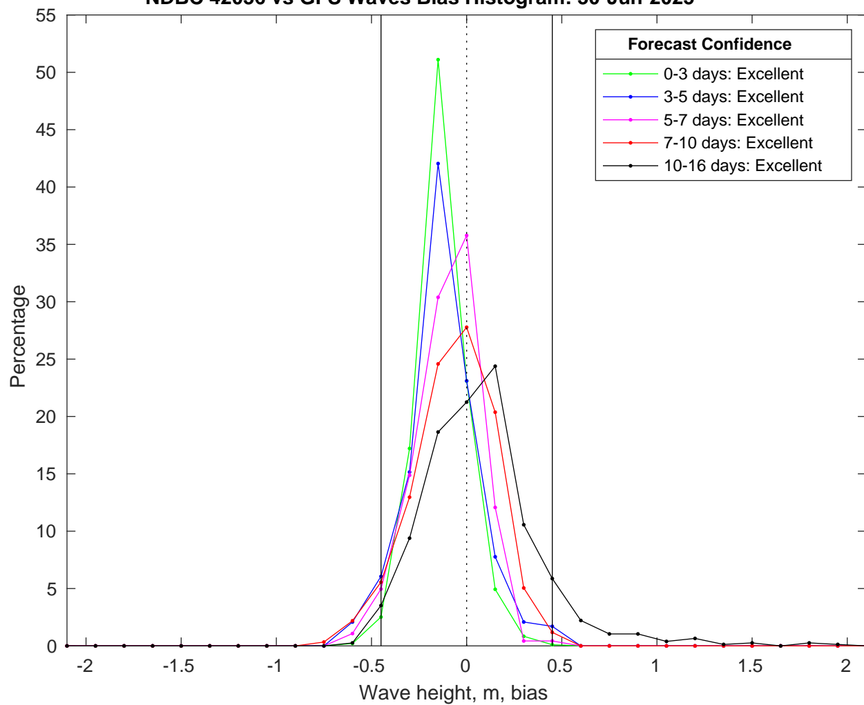
NDBC 42036 vs GFS Waves Bias Histogram: 30-Jun-2025
