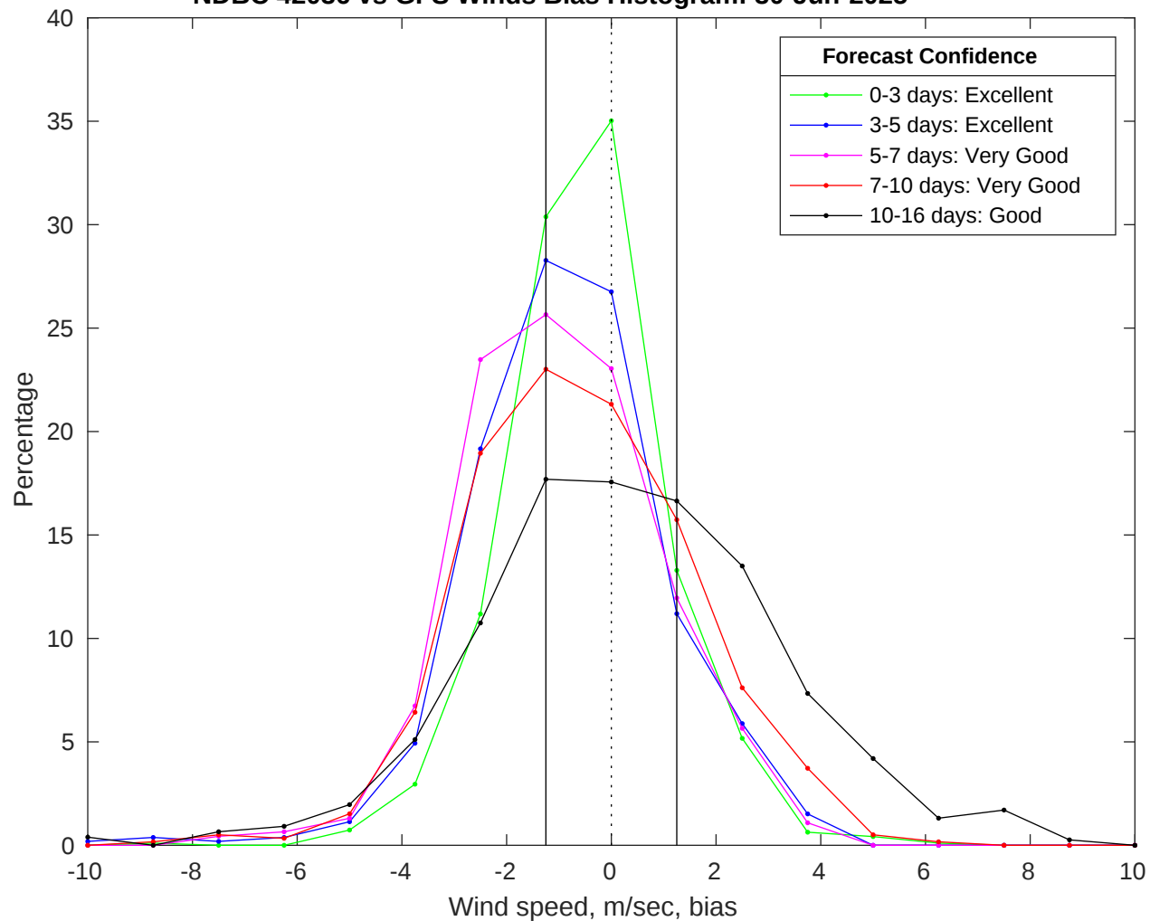
NDBC 42036 vs GFS Winds Bias Histogram: 30-Jun-2025
