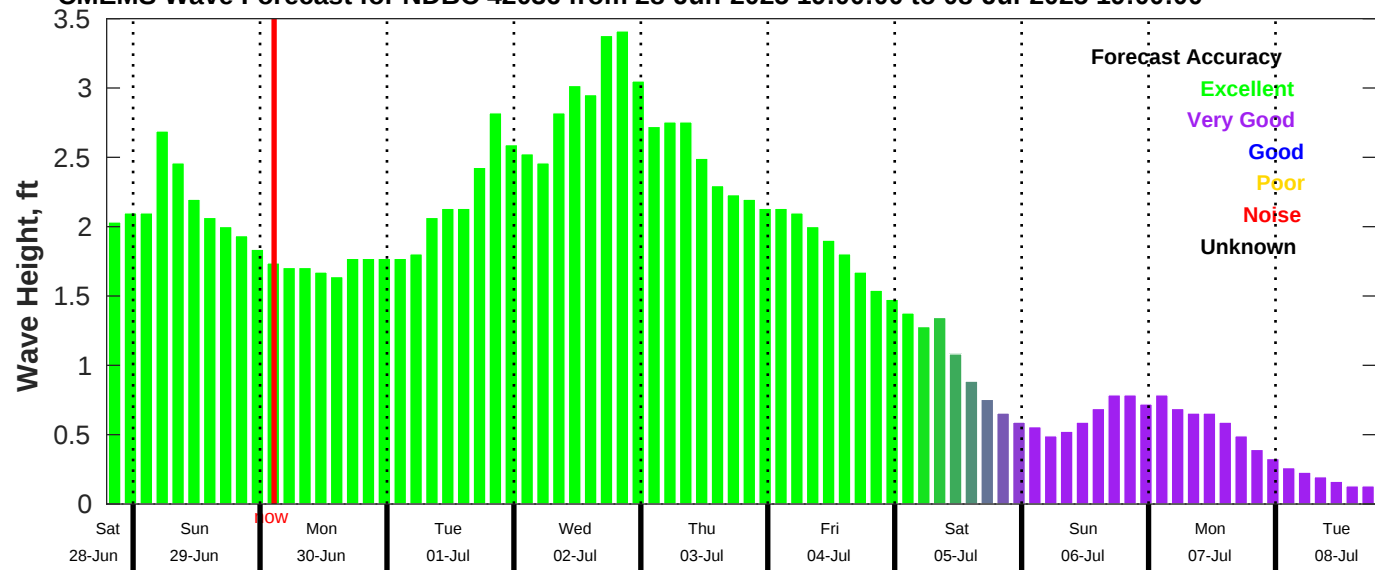
CMEMS Wave Forecast for NDBC 42036 from 28-Jun-2025 19:00:00 to 08-Jul-2025 19:00:00
