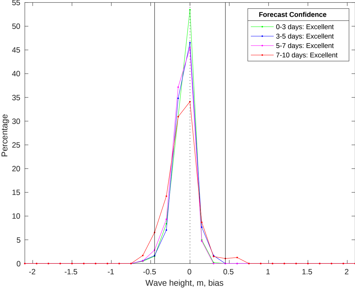
NDBC 42040 vs CMEMS Waves Bias Histogram: 30-Jun-2025
