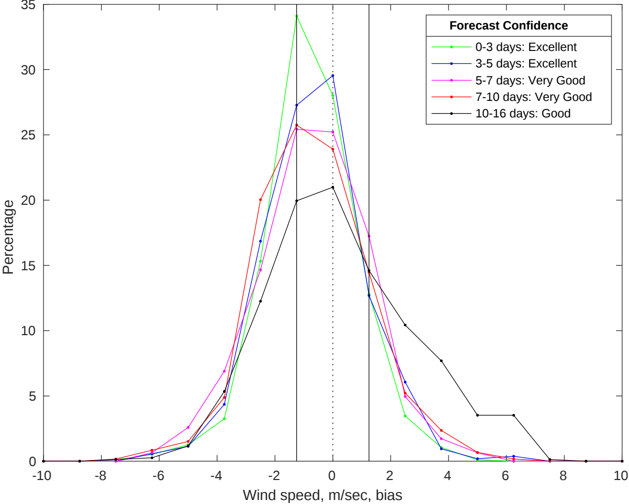
NDBC 42040 vs GFS Winds Bias Histogram: 30-Jun-2025
