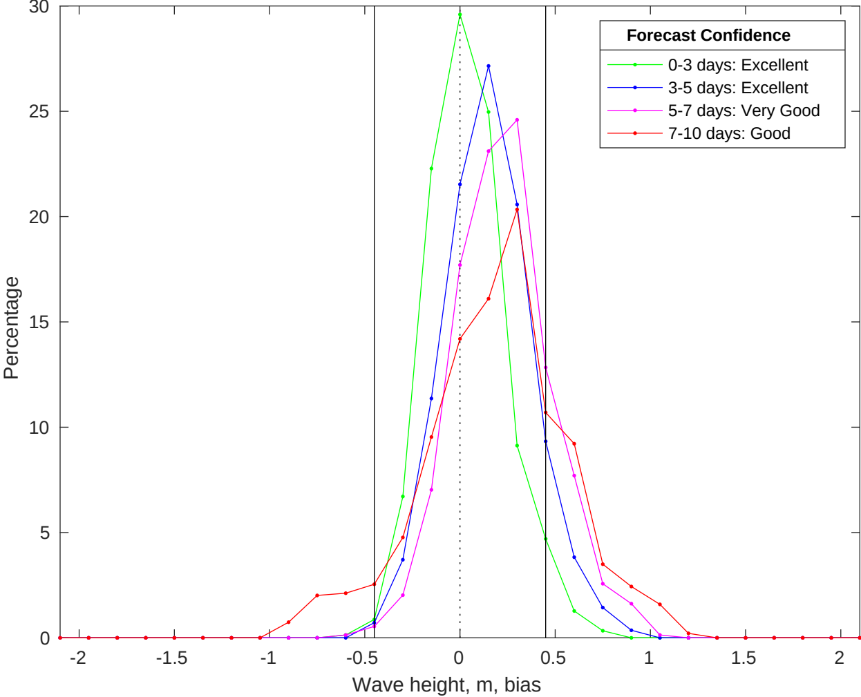
NDBC 46011 vs CMEMS Waves Bias Histogram: 30-Jun-2025
