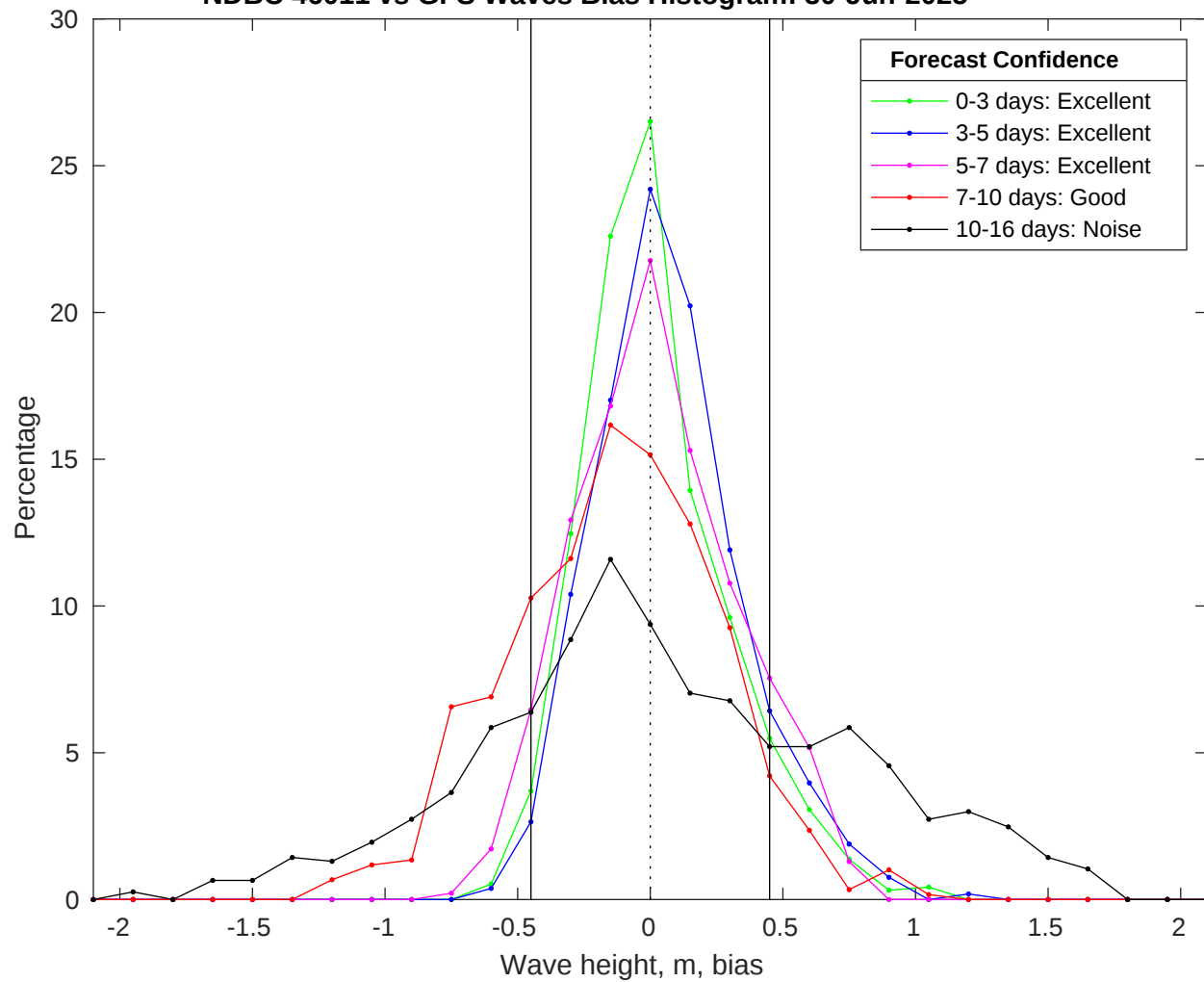
NDBC 46011 vs GFS Waves Bias Histogram: 30-Jun-2025
