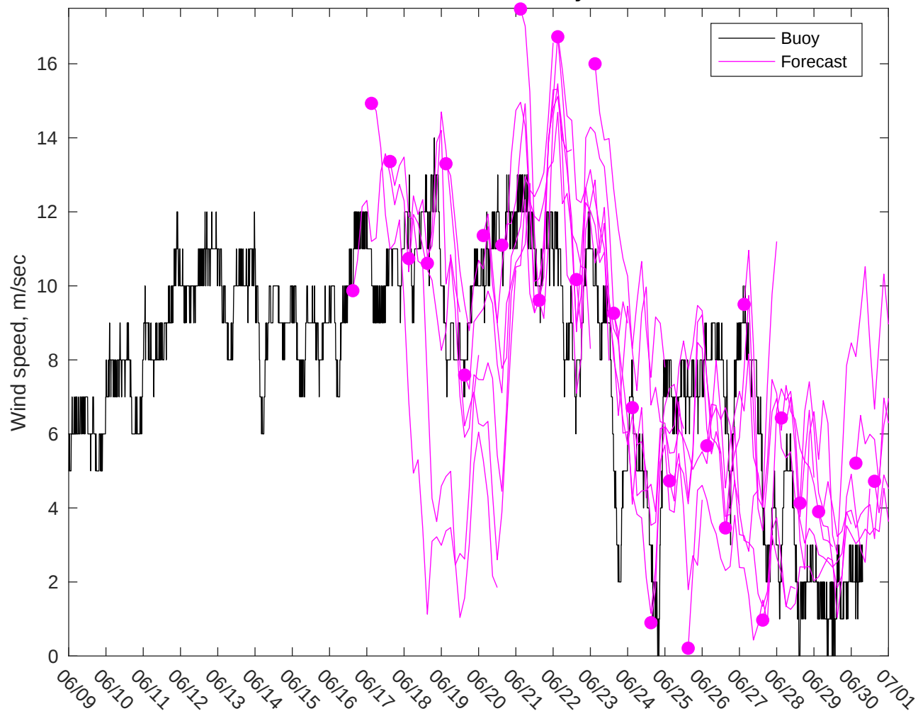
NDBC 46011 vs GFS Winds: 7 to 10 day forecast
