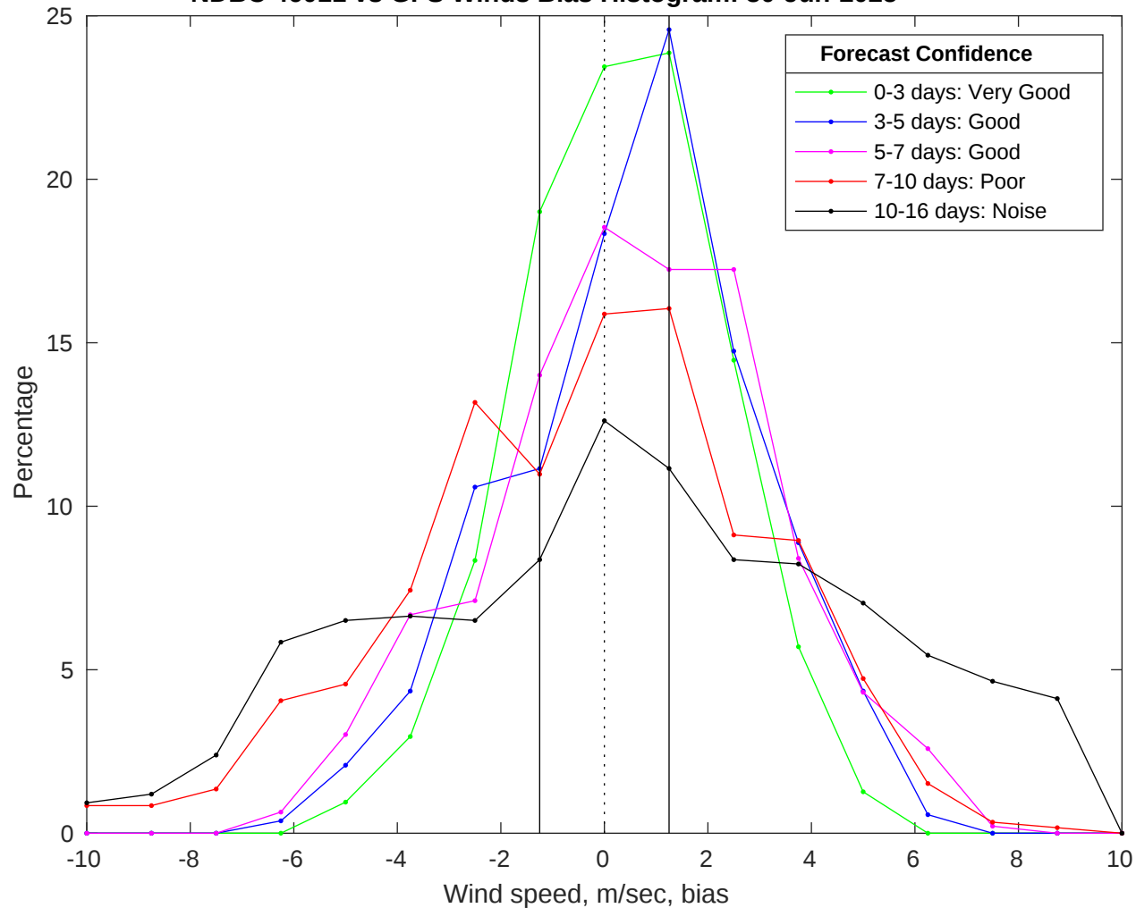
NDBC 46011 vs GFS Winds Bias Histogram: 30-Jun-2025
