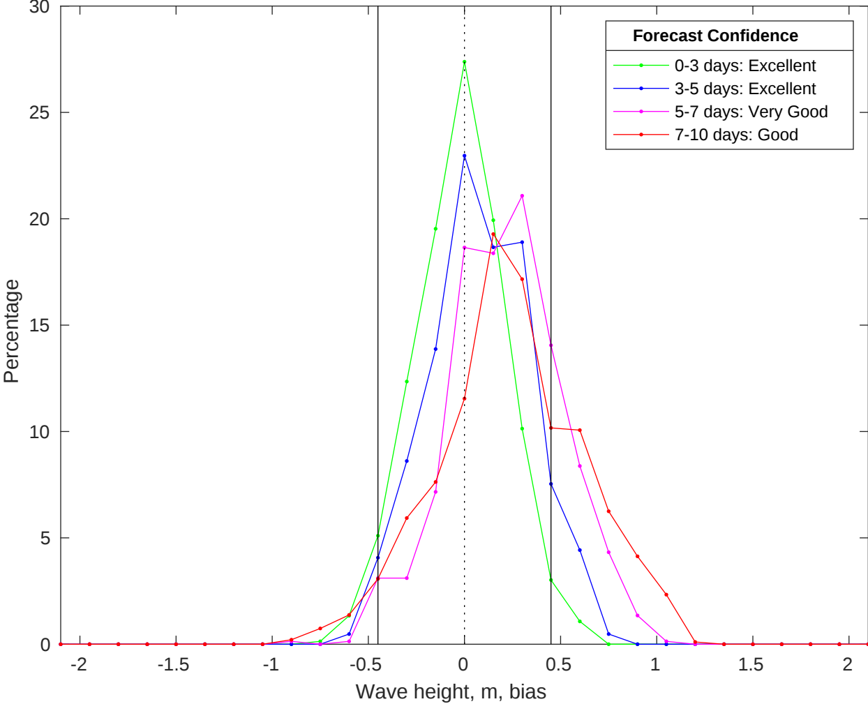
NDBC 46028 vs CMEMS Waves Bias Histogram: 30-Jun-2025
