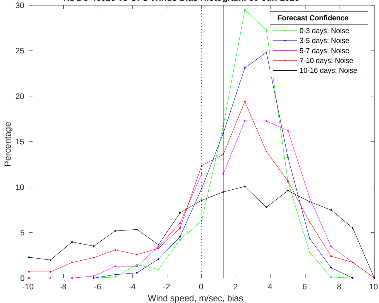
NDBC 46028 vs GFS Winds Bias Histogram: 30-Jun-2025
