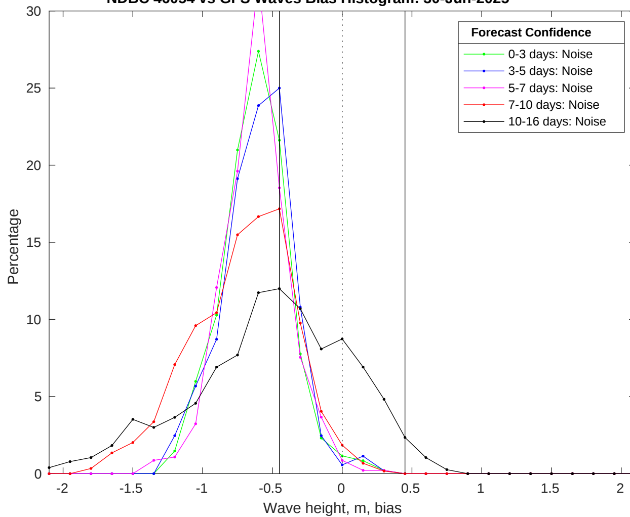
NDBC 46054 vs GFS Waves Bias Histogram: 30-Jun-2025
