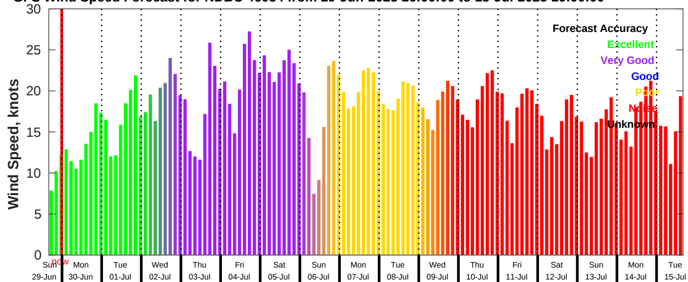
GFS Wind Speed Forecast for NDBC 46054 from 29-Jun-2025 16:00:00 to 15-Jul-2025 16:00:00
