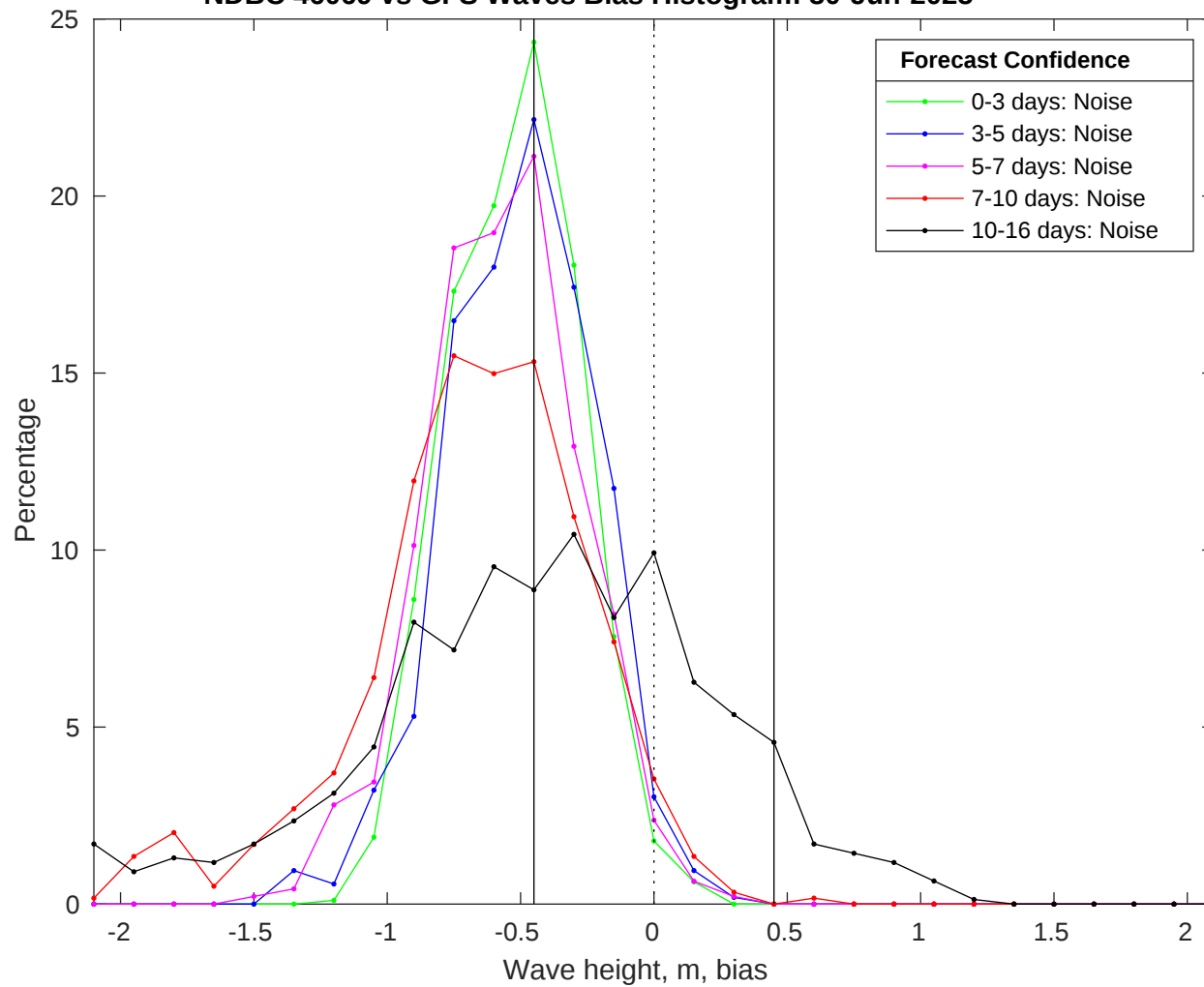
NDBC 46069 vs GFS Waves Bias Histogram: 30-Jun-2025
