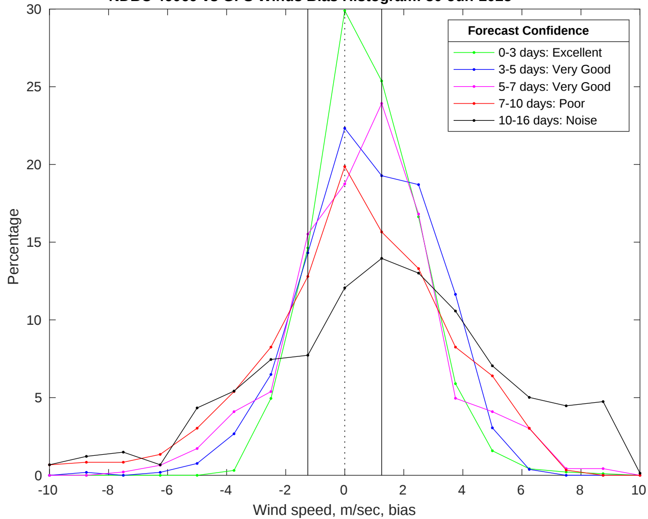
NDBC 46069 vs GFS Winds Bias Histogram: 30-Jun-2025
