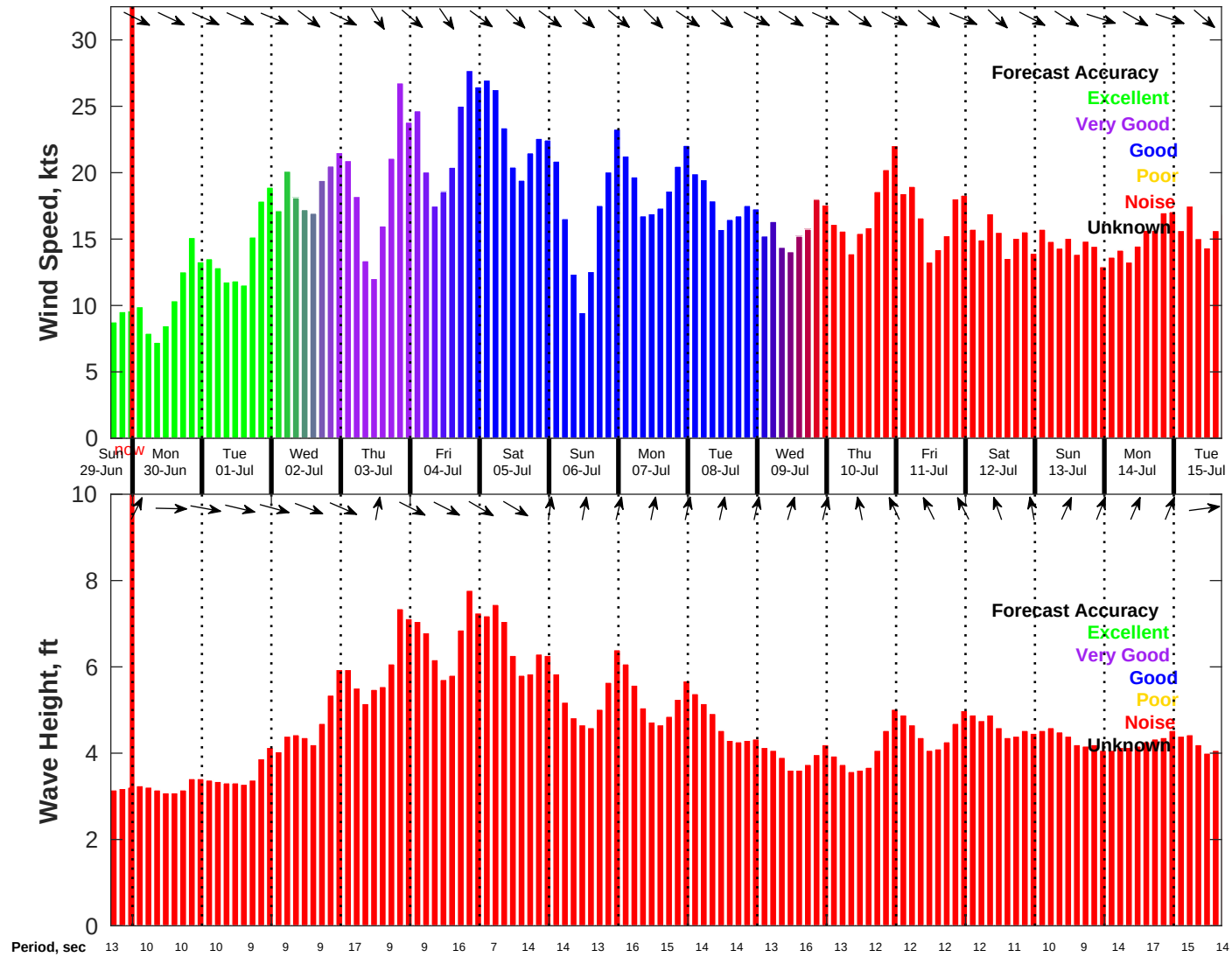
Wind & Wave Forecast for NDBC 46069 from 29-Jun-2025 16:00:00 to 15-Jul-2025 16:00:00
