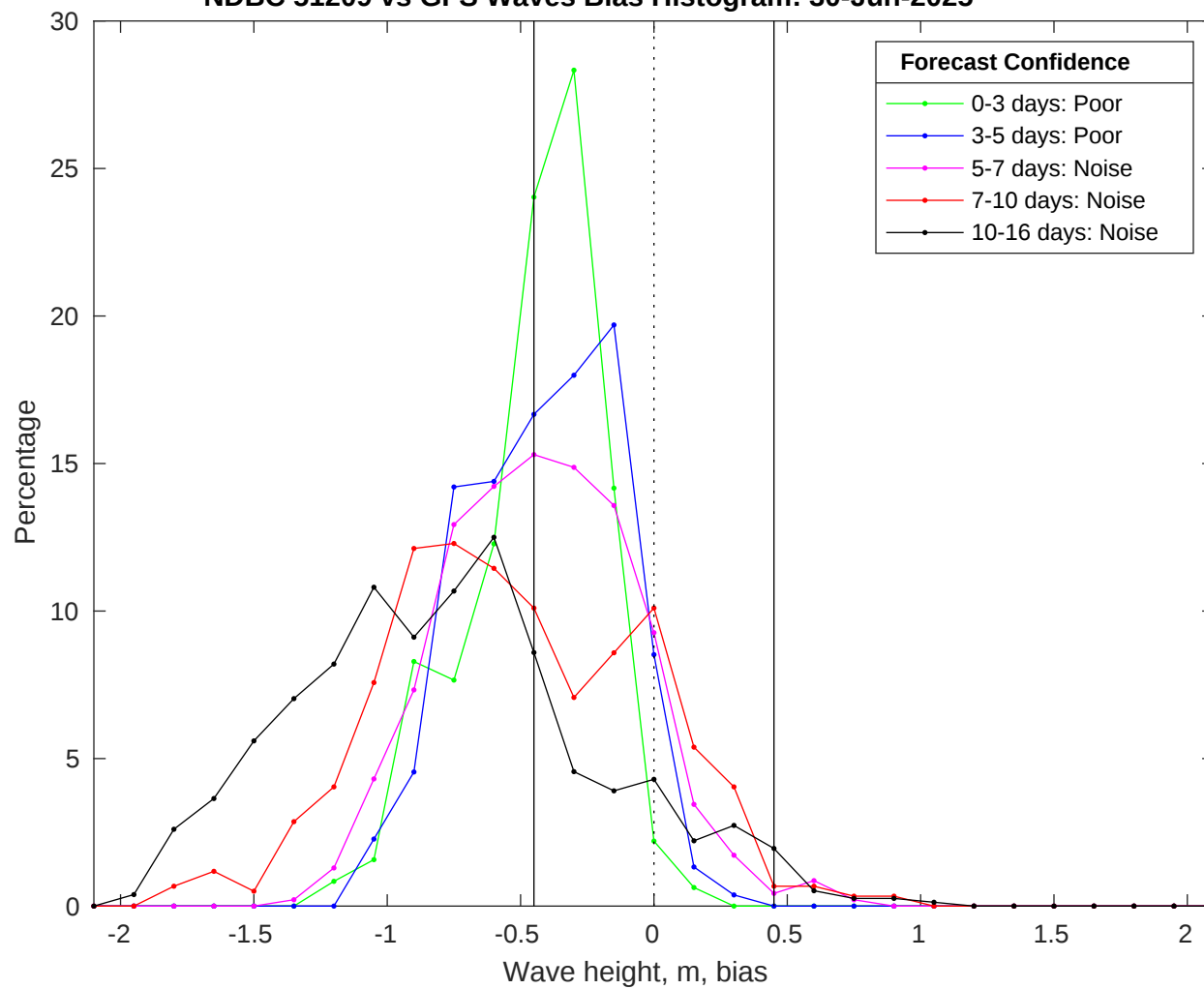
NDBC 51209 vs GFS Waves Bias Histogram: 30-Jun-2025
