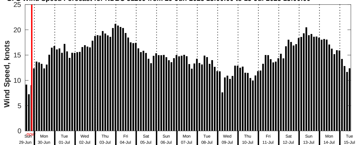
GFS Wind Speed Forecast for NDBC 51209 from 29-Jun-2025 13:00:00 to 15-Jul-2025 13:00:00
