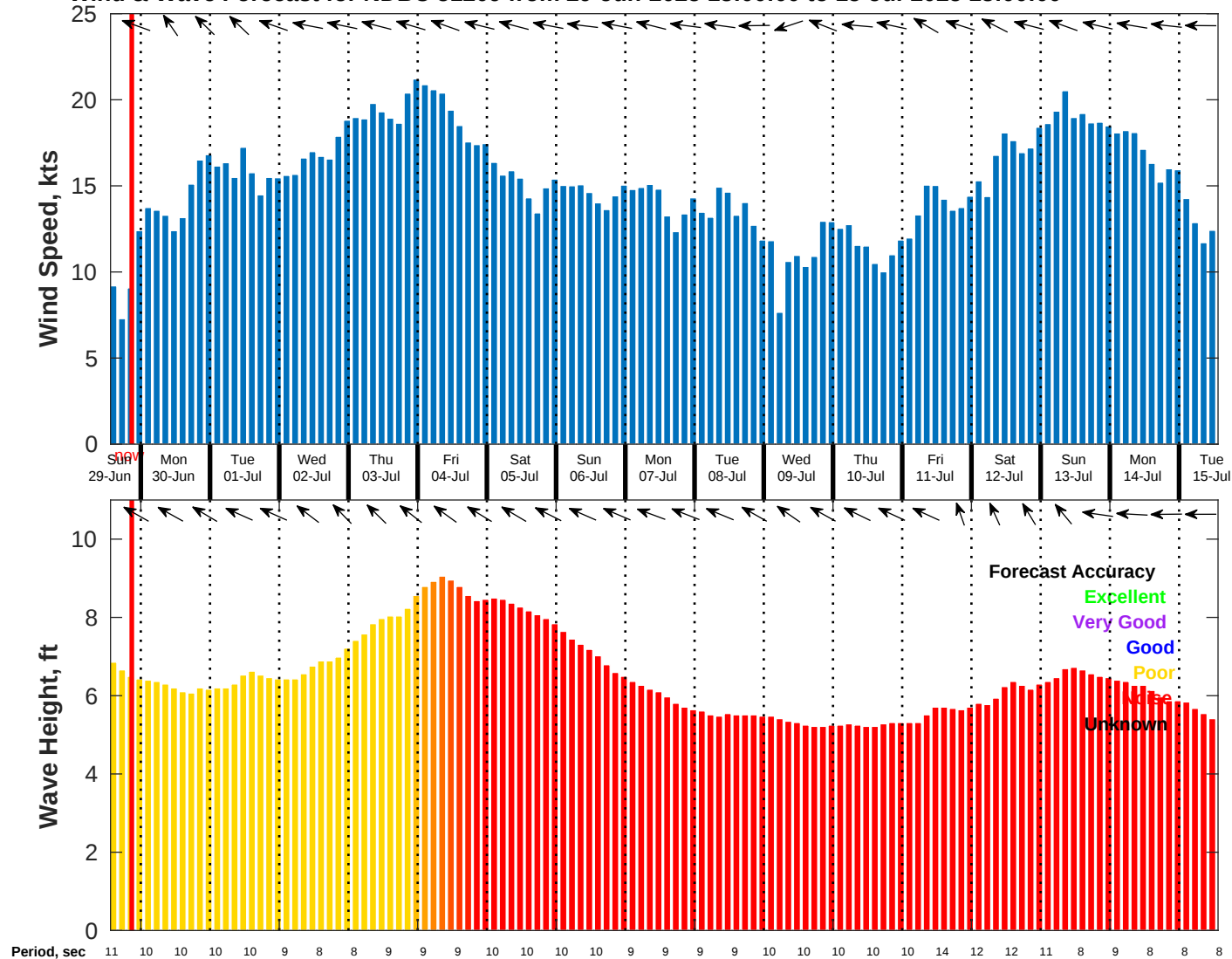
Wind & Wave Forecast for NDBC 51209 from 29-Jun-2025 13:00:00 to 15-Jul-2025 13:00:00
