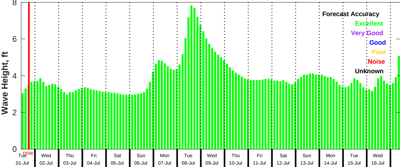
GFS Wave Forecast for NDBC 52211 from 30-Jun-2025 10:00:00 to 16-Jul-2025 10:00:00
