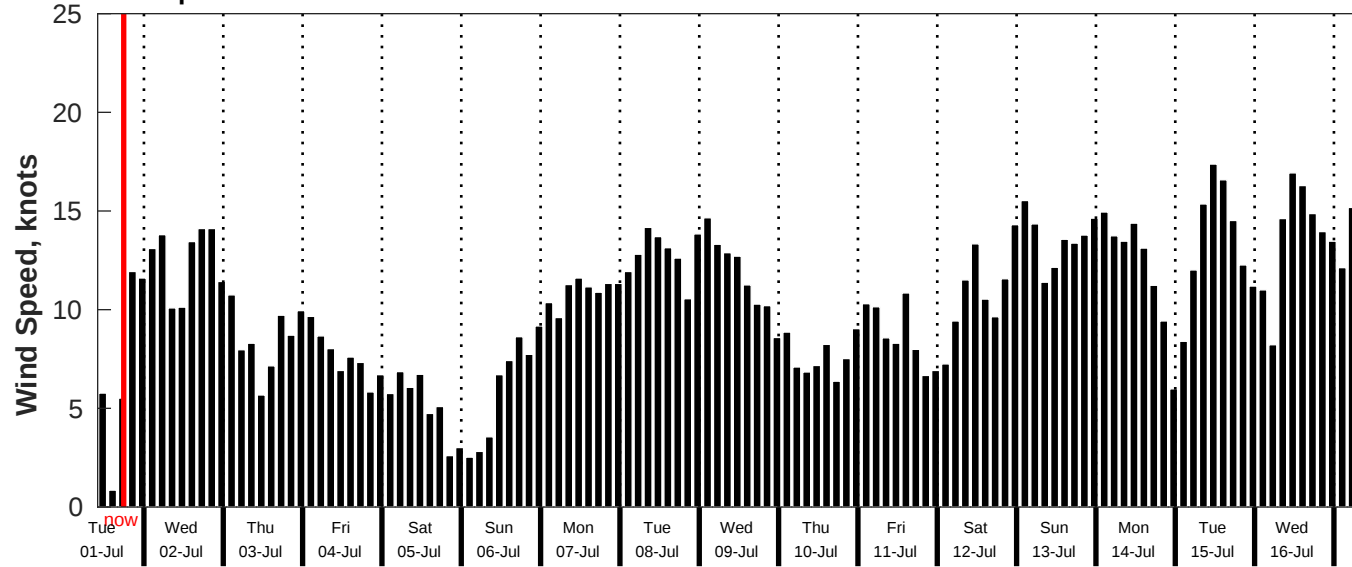
GFS Wind Speed Forecast for NDBC 52211 from 30-Jun-2025 10:00:00 to 16-Jul-2025 10:00:00
