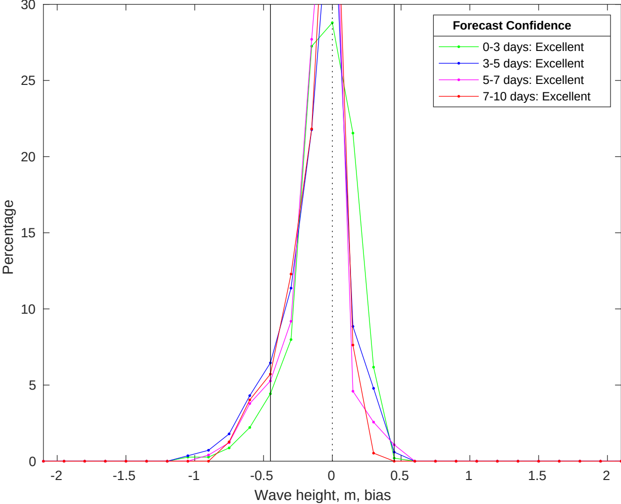
NDBC 52212 vs CMEMS Waves Bias Histogram: 30-Jun-2025
