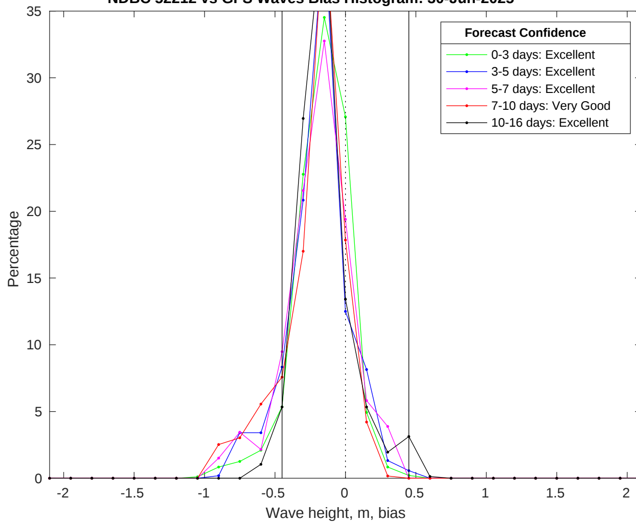
NDBC 52212 vs GFS Waves Bias Histogram: 30-Jun-2025
