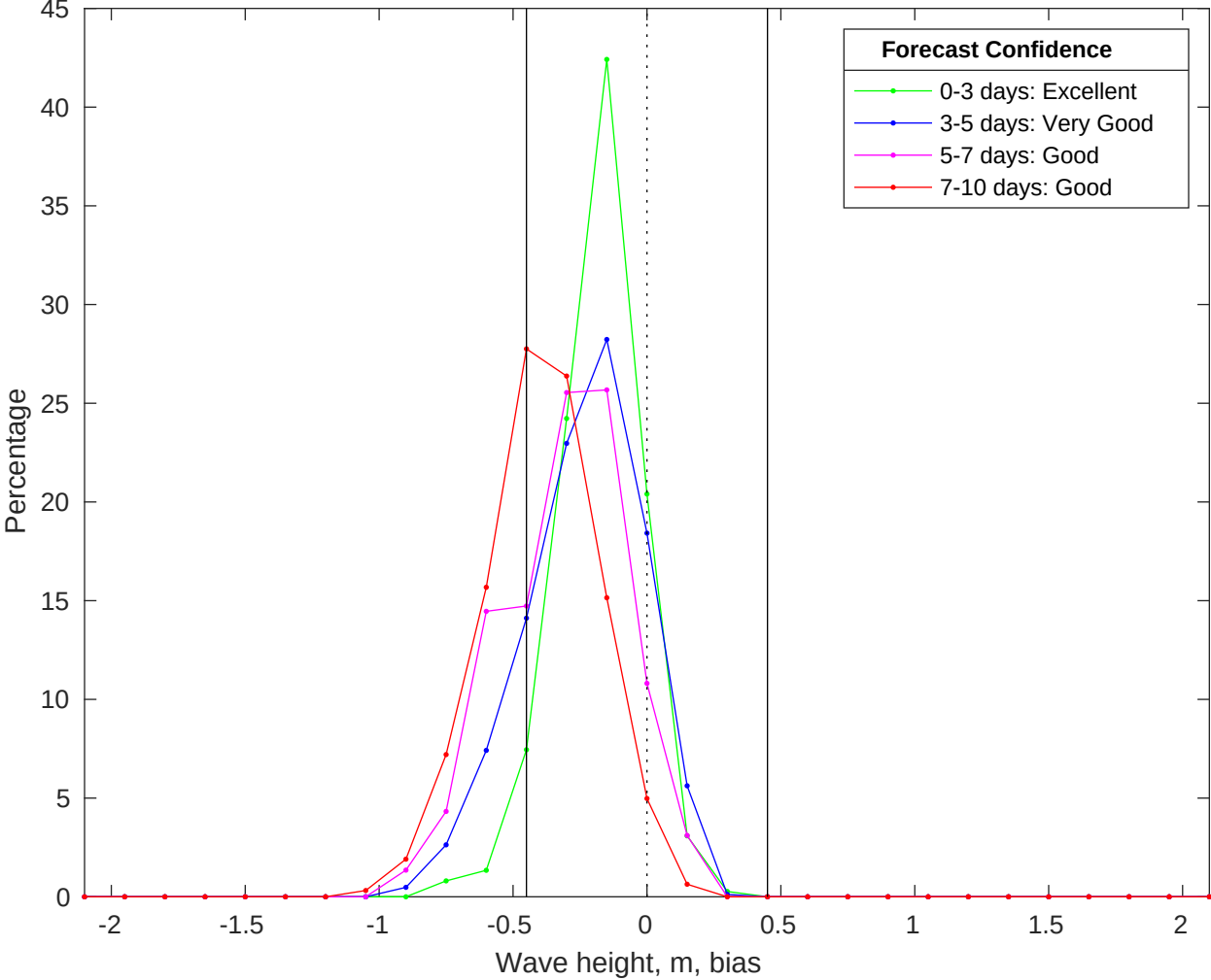
NDBC 52213 vs CMEMS Waves Bias Histogram: 30-Jun-2025
