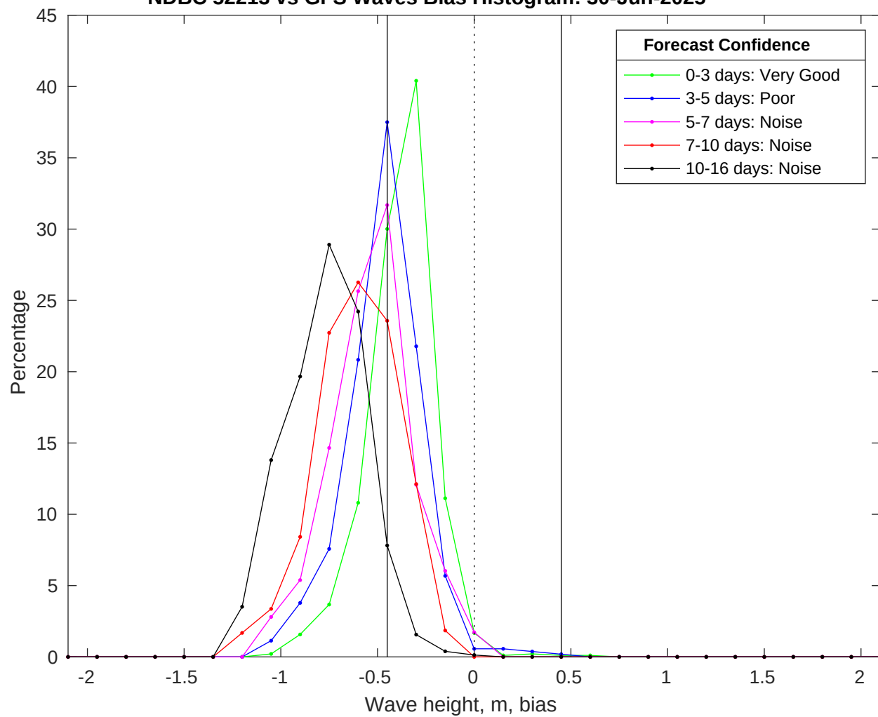
NDBC 52213 vs GFS Waves Bias Histogram: 30-Jun-2025
