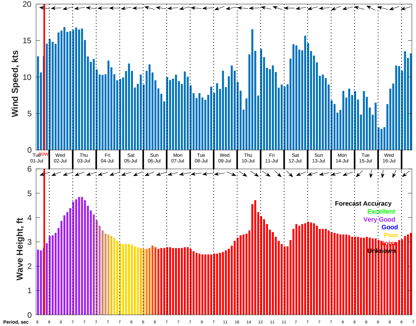
Wind & Wave Forecast for NDBC 52213 from 30-Jun-2025 11:00:00 to 16-Jul-2025 11:00:00
